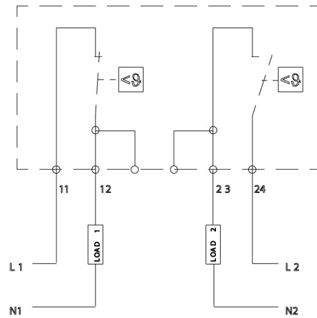
CONNECTION DIAGRAM
